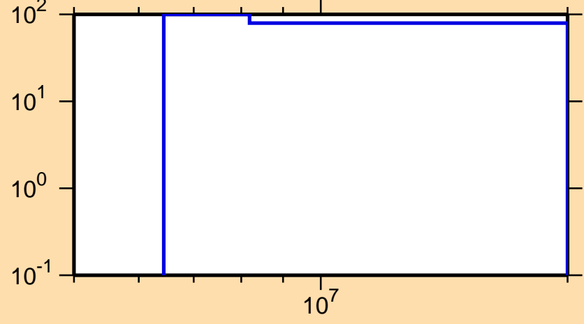
\Delta\sigma/\sigma vs. E for ^{162}\text{Lu}(n,2n)
