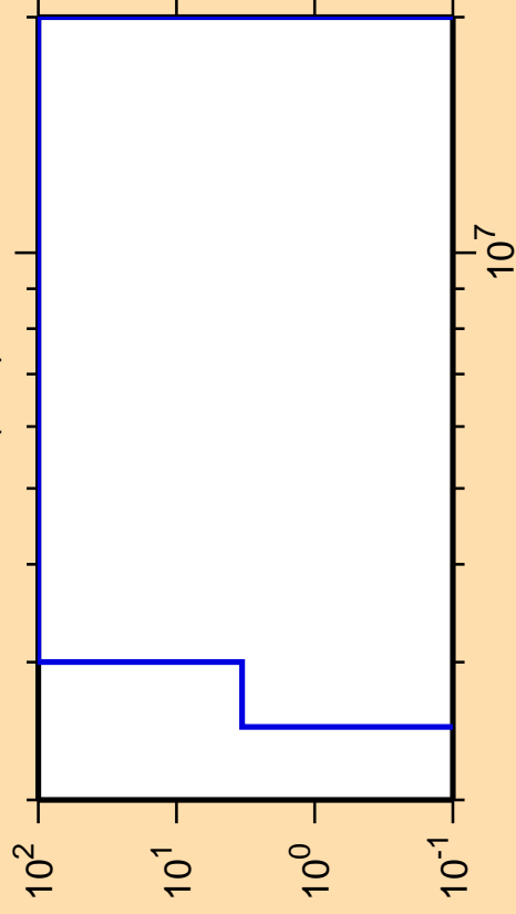
\Delta\sigma/\sigma vs. E for ^{162}\text{Lu}(n,d)
