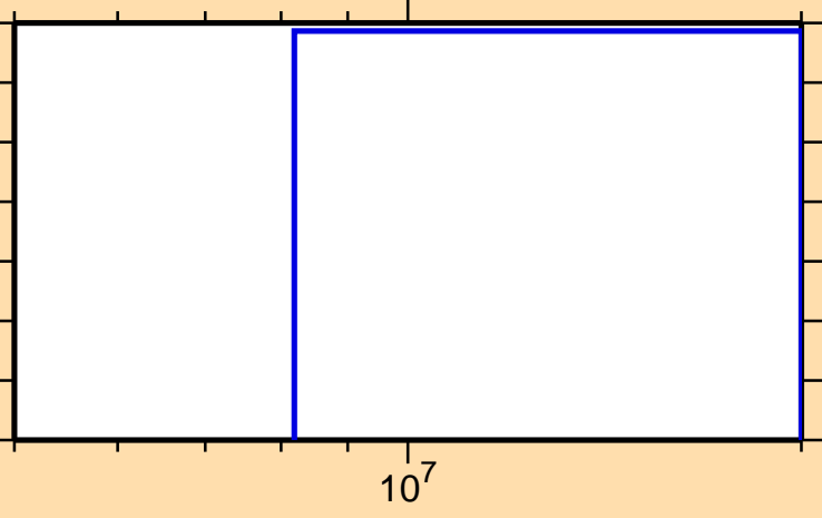
\sigma vs. E for ^{162}\text{Lu}(n,2np)
