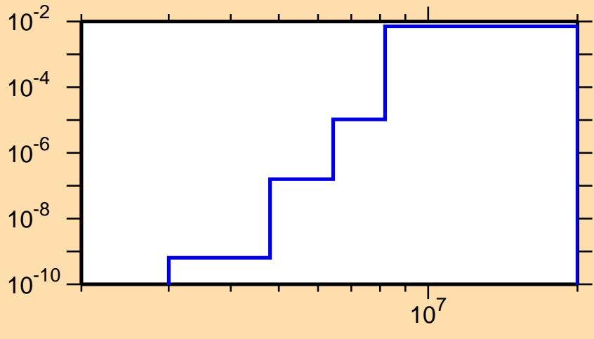
\sigma vs. E for ^{162}\text{Lu}(n,d)
