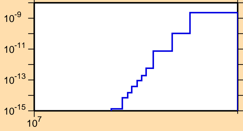
\sigma vs. E for ^{162}\text{Lu} (mt 34)
