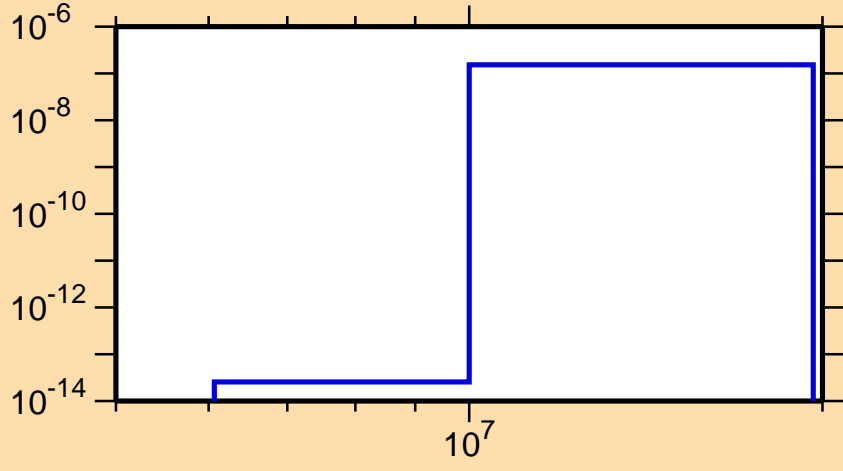
\sigma vs. E for ^{163}\text{Lu} (mt 45)
