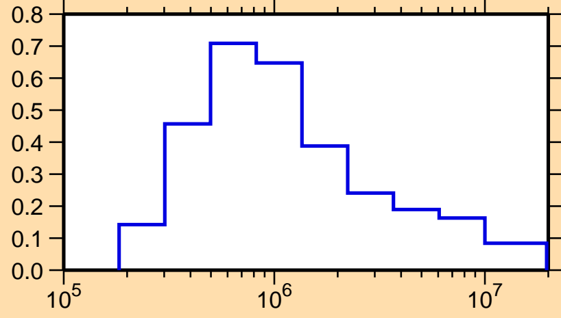
\sigma vs. E for ^{163}\text{Lu}(n,n_4)
