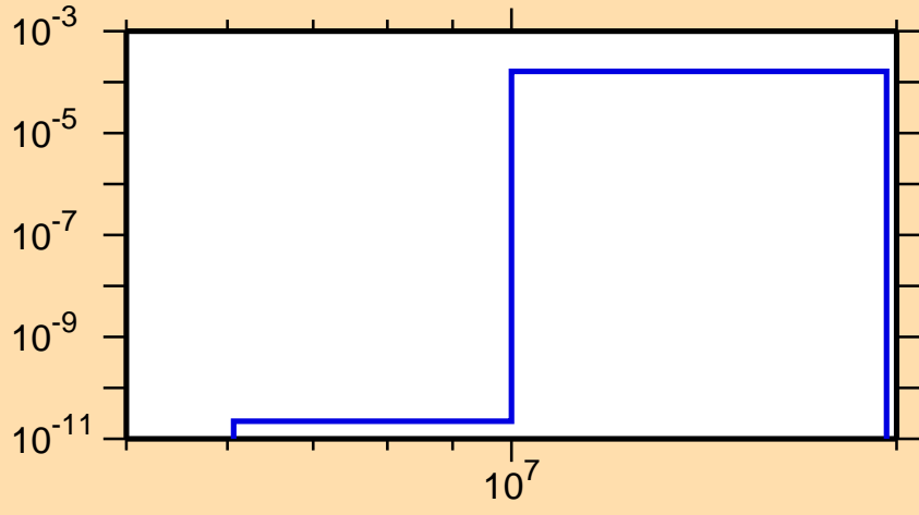
\sigma vs. E for ^{163}\text{Lu}(n,t)
