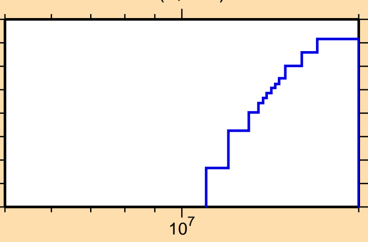
\sigma vs. E for ^{164}\text{Lu}(n,2n\alpha)
