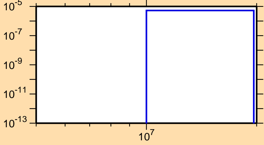
\sigma vs. E for ^{164}\text{Lu}(n,\text{nd})
