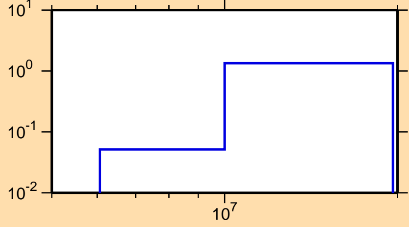
\sigma vs. E for ^{164}\text{Lu}(n,2n)
