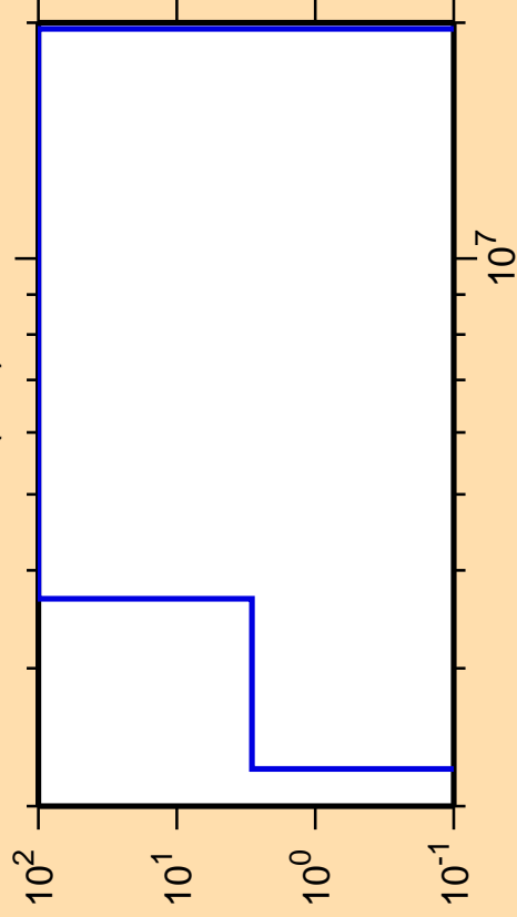
\Delta\sigma/\sigma vs. E for ^{164}\text{Lu}(n,d)
