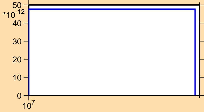
\sigma vs. E for ^{164}\text{Lu}(n,pt)
