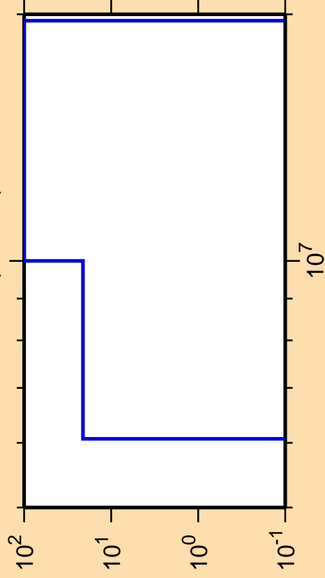
\Delta\sigma/\sigma vs. E for ^{164}\text{Lu}(n,\text{He}3)
