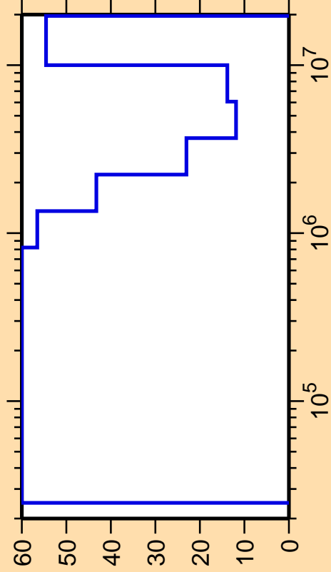
\Delta\sigma/\sigma vs. E for ^{164}\text{Lu}(n,\text{inel.})
