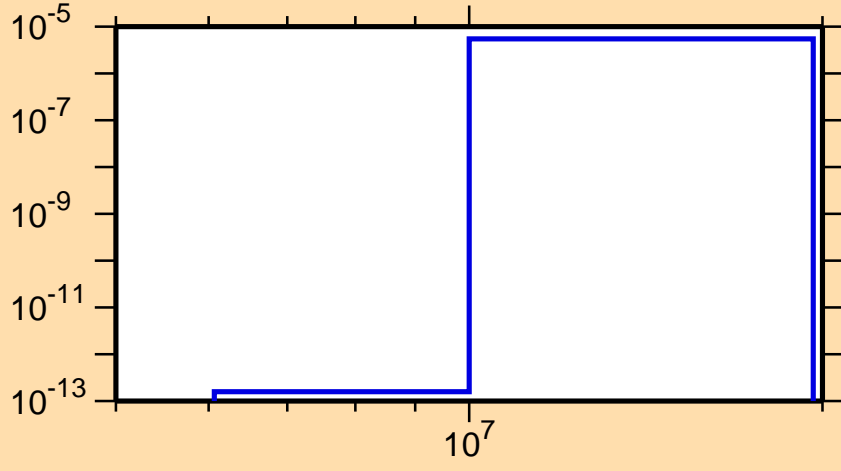
\sigma vs. E for ^{164}\text{Lu}(n,2n\alpha)
