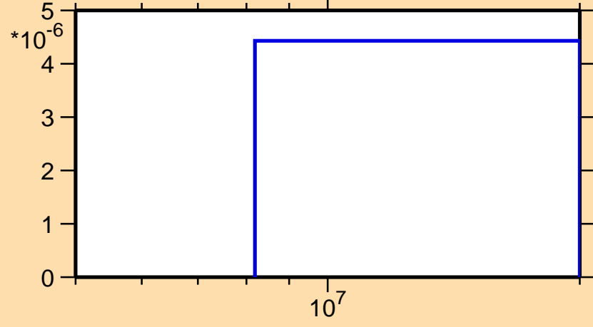
\sigma vs. E for ^{164}\text{Lu}(n,2n\alpha)
