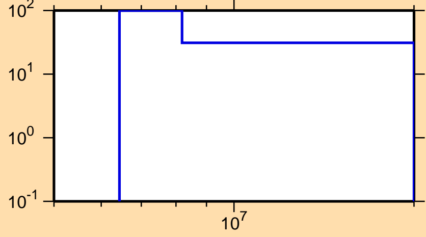
\Delta\sigma/\sigma vs. E for ^{164}\text{Lu}(n,2n)
