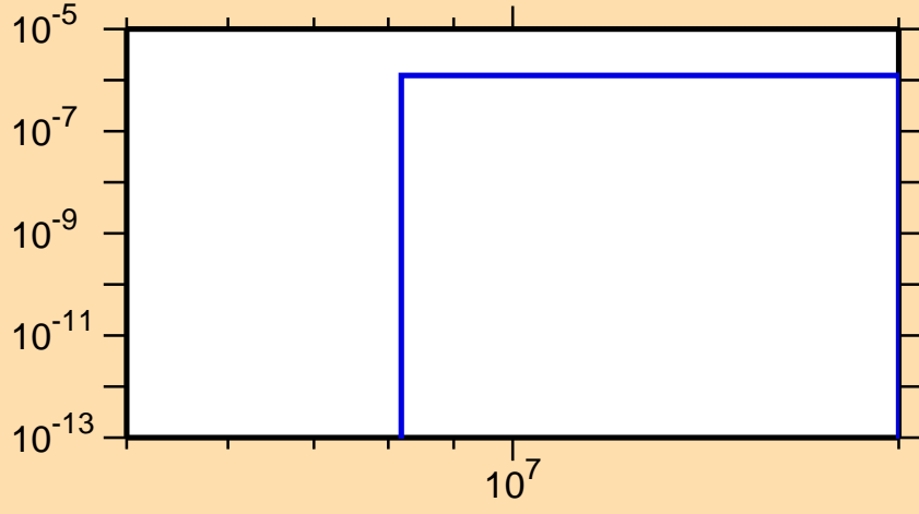
\sigma vs. E for ^{164}\text{Lu}(n,\text{He3})
