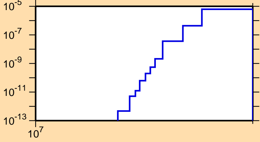
\sigma vs. E for ^{165}\text{Lu}(n,nd)
