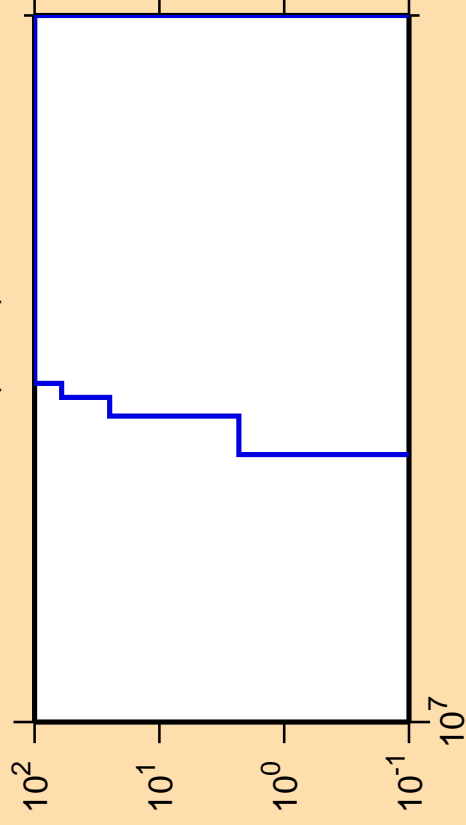
\Delta\sigma/\sigma vs. E for ^{165}\text{Lu}(n,nd)
