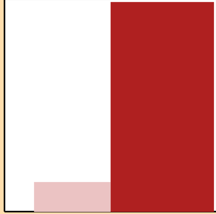
\Delta\sigma/\sigma vs. E for ^{165}\text{Lu}(n,2n)
