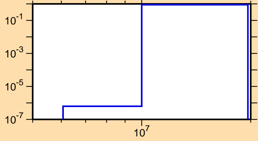
\sigma vs. E for ^{165}\text{Lu}(n,2n)
