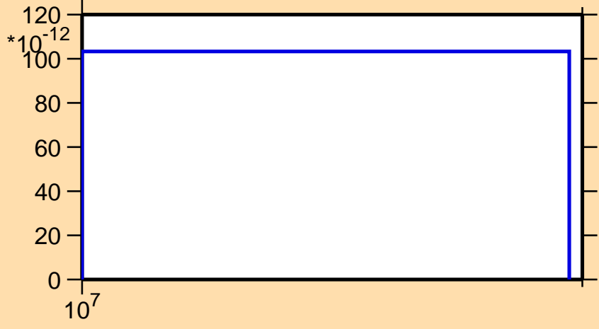
\sigma vs. E for ^{165}\text{Lu}(n,pd)
