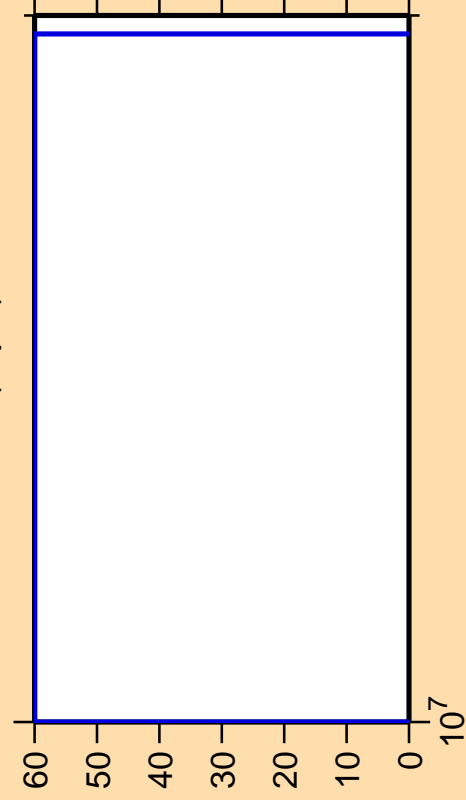
\Delta\sigma/\sigma vs. E for ^{165}\text{Lu}(n,pd)
