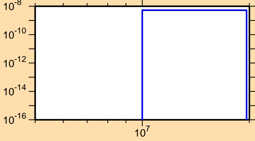
\sigma vs. E for ^{165}\text{Lu} (mt 45)
