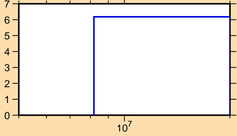
\Delta\sigma/\sigma vs. E for ^{165}\text{Lu}(n,\text{el.})
