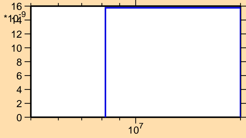
\sigma vs. E for ^{165}\text{Lu}(n,2n\alpha)
