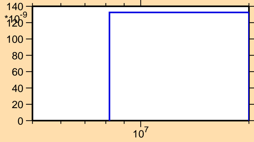
\sigma vs. E for ^{165}\text{Lu}(n,\text{He}3)
