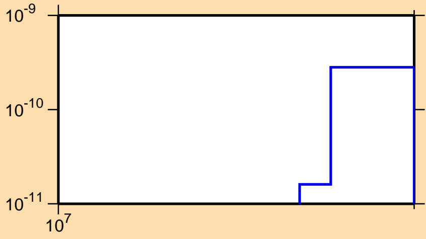
\sigma vs. E for ^{166}\text{Lu}(n,pd)
