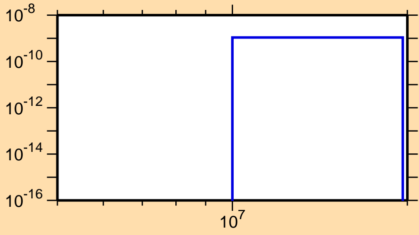
\sigma vs. E for ^{166}\text{Lu} (mt 45)
