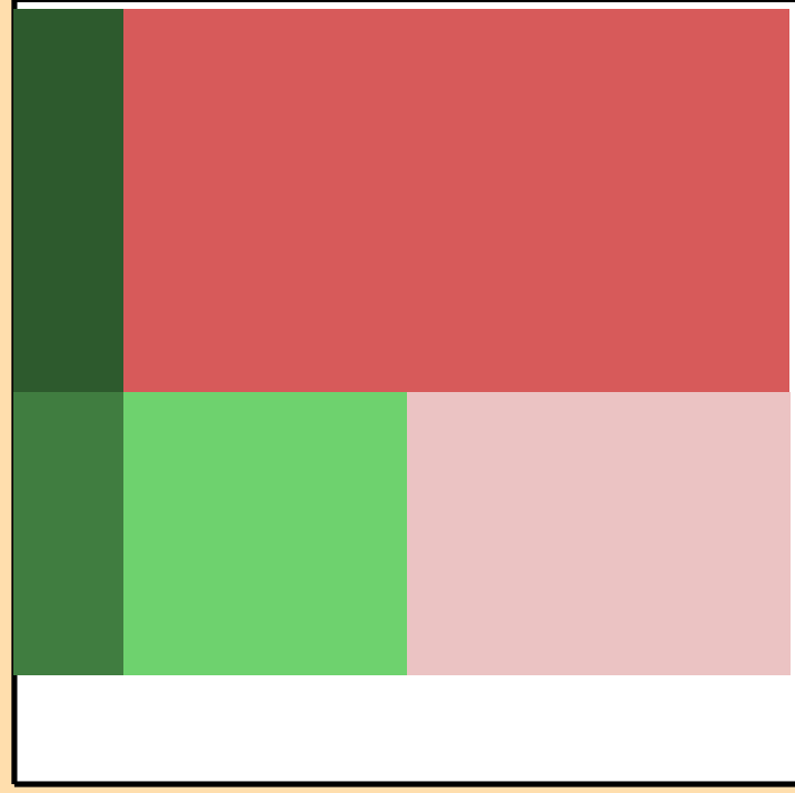
\Delta\sigma/\sigma vs. E for ^{166}\text{Lu}(n,\text{tot.})
