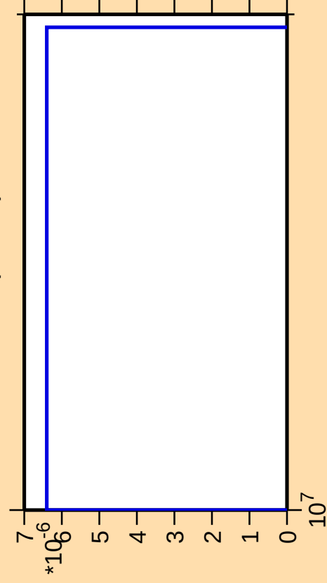
\Delta\sigma/\sigma vs. E for ^{166}\text{Lu}(\text{mt 11})
