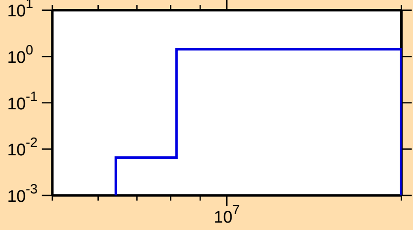
\sigma vs. E for ^{166}\text{Lu}(n,2n)
