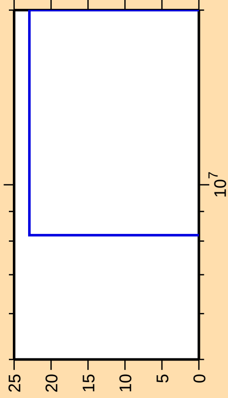
\Delta\sigma/\sigma vs. E for ^{166}\text{Lu}(\text{mt } 34)
