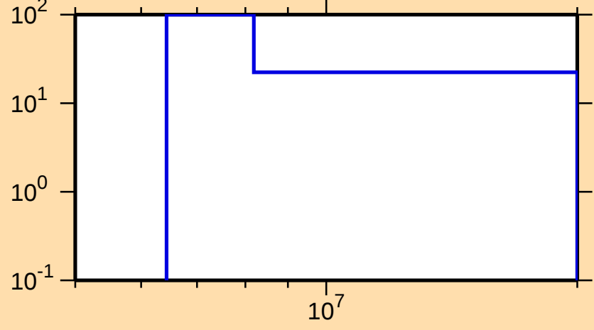
\Delta\sigma/\sigma vs. E for ^{166}\text{Lu}(n,2n)
