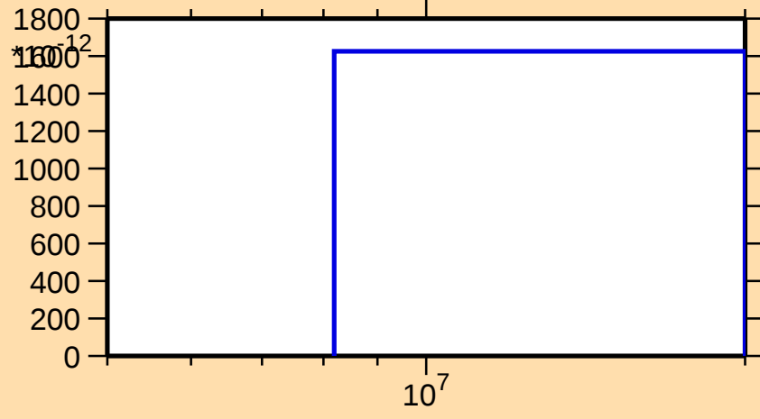
\sigma vs. E for ^{166}\text{Lu}(\text{mt } 45)
