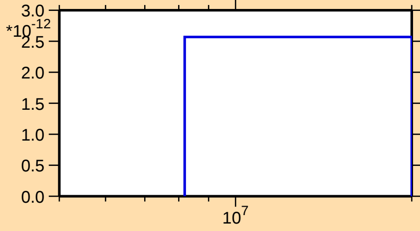
\sigma vs. E for ^{166}\text{Lu}(\text{mt } 34)
