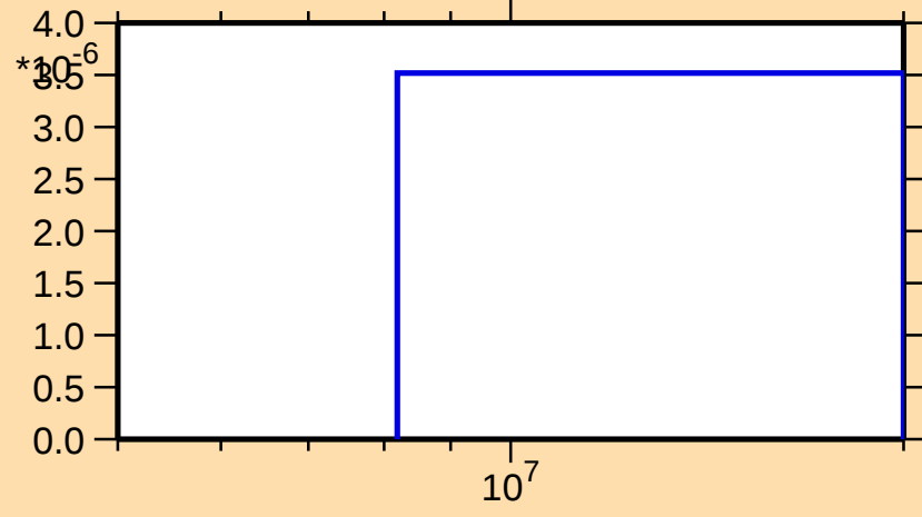
\sigma vs. E for ^{166}\text{Lu}(n,2n\alpha)
