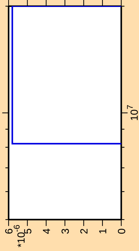
\Delta\sigma/\sigma vs. E for ^{166}\text{Lu}(\text{mt 11})
