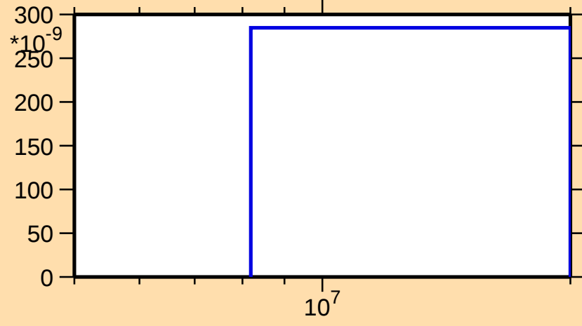
\sigma vs. E for ^{166}\text{Lu}(n,\text{He3})
