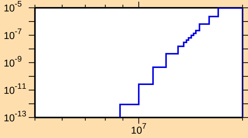
\sigma vs. E for ^{166}\text{Lu}(n,\text{He3})
