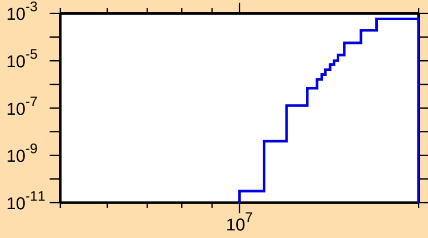
\sigma vs. E for ^{166}\text{Lu}(n,2n\alpha)
