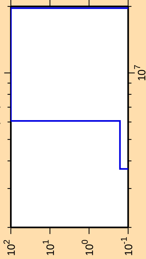
\Delta\sigma/\sigma vs. E for ^{166}\text{Lu}(n,t)
