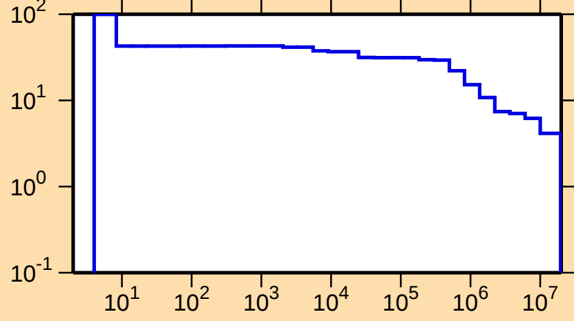
\Delta\sigma/\sigma vs. E for ^{166}\text{Lu}(n,\text{nonel.})
