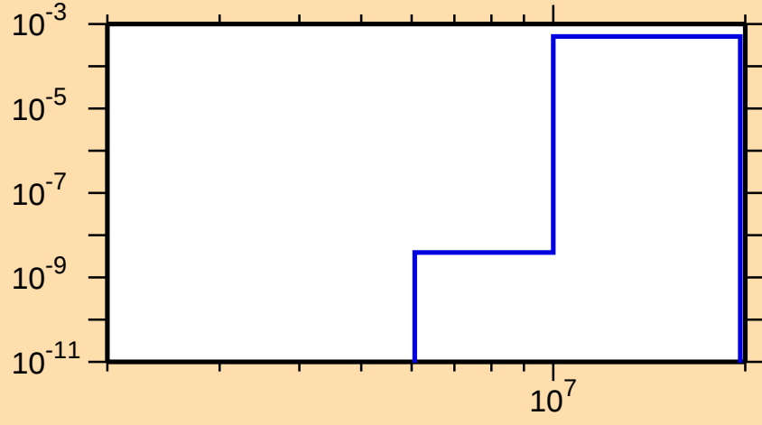
\sigma vs. E for ^{166}\text{Lu}(n,t)
