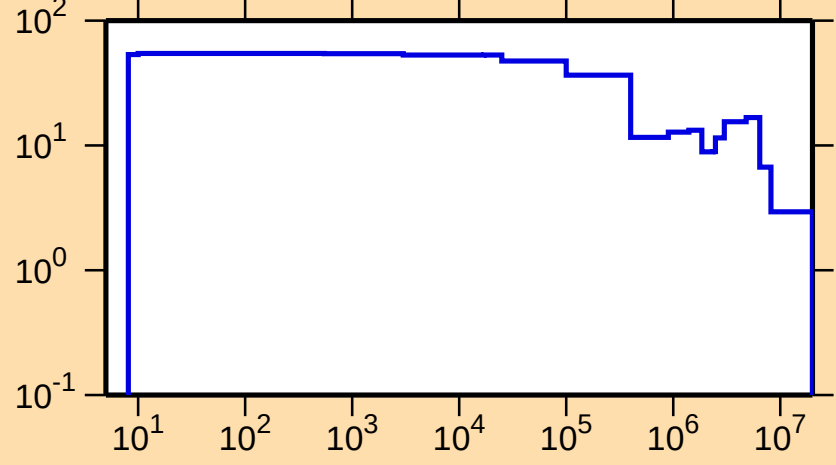
\Delta\sigma/\sigma vs. E for ^{166}\text{Lu}(n,\text{el.})
