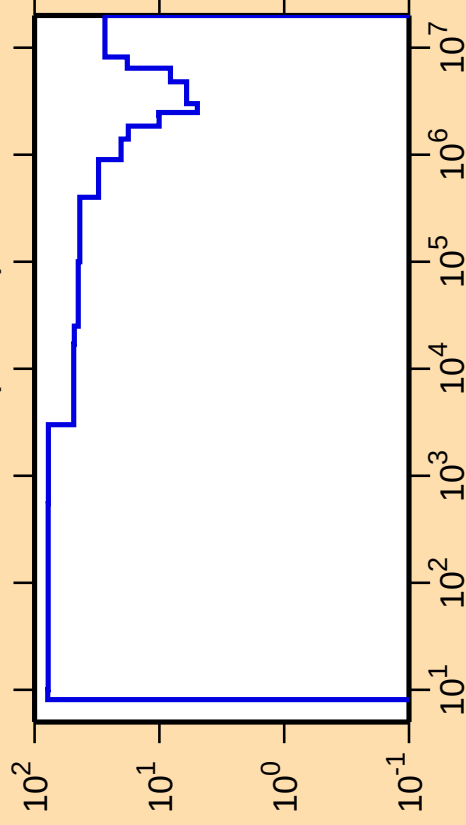
\Delta\sigma/\sigma vs. E for ^{166}\text{Lu}(n,\text{inel.})
