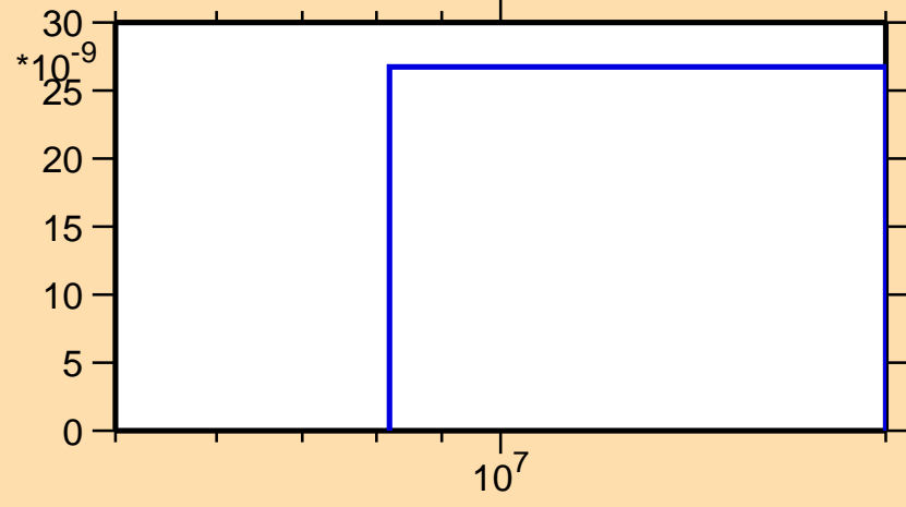
\sigma vs. E for ^{167}\text{Lu}(n,\text{He3})
