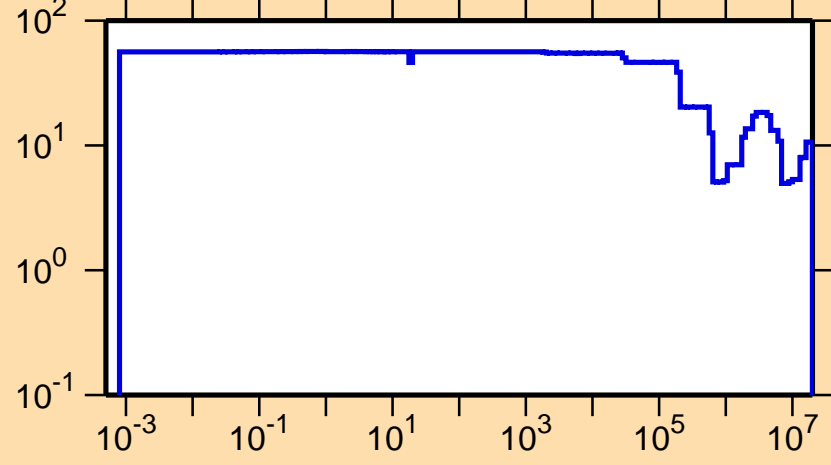
\Delta\sigma/\sigma vs. E for ^{167}\text{Lu}(n,\text{el.})
