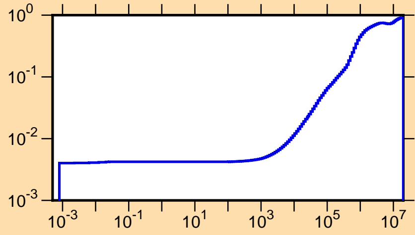
\mu vs. E for ^{168}\text{Lu}(\text{mt251})
