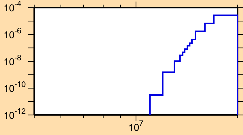
\sigma vs. E for ^{168}\text{Lu}(n,2n\alpha)
