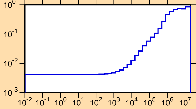
\mu vs. E for ^{168}\text{Lu}(\text{mt251})
