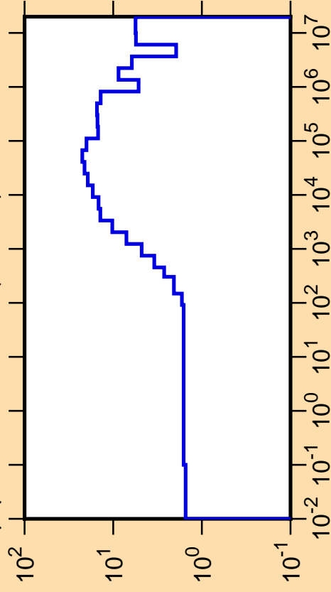
\Delta\mu/\mu vs. E for ^{168}\text{Lu}(\text{mt251})
