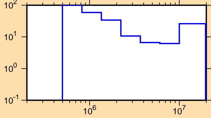
\Delta\sigma/\sigma vs. E for ^{168}\text{Lu}(n,n\text{cont.})
