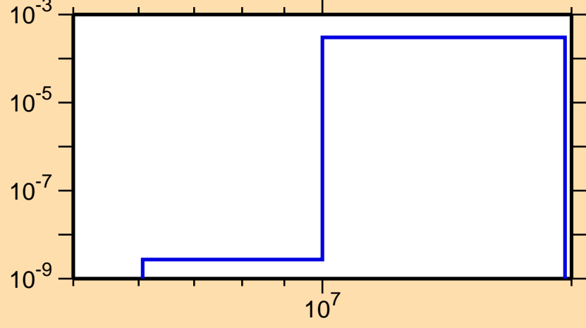
\sigma vs. E for ^{168}\text{Lu}(n,t)
