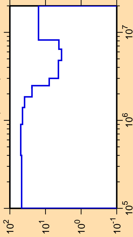
\Delta\sigma/\sigma vs. E for ^{168}\text{Lu}(n,\text{inel.})
