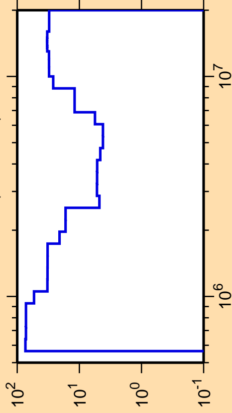
\Delta\sigma/\sigma vs. E for ^{168}\text{Lu}(n,n\text{cont.})
