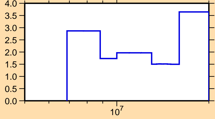
\Delta\sigma/\sigma vs. E for ^{168}\text{Lu}(n,\text{tot.})
