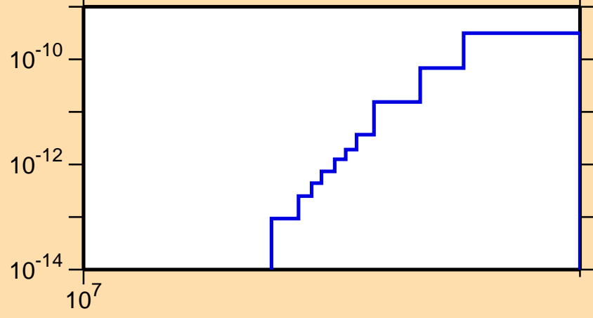
\sigma vs. E for ^{168}\text{Lu}(\text{mt117})
