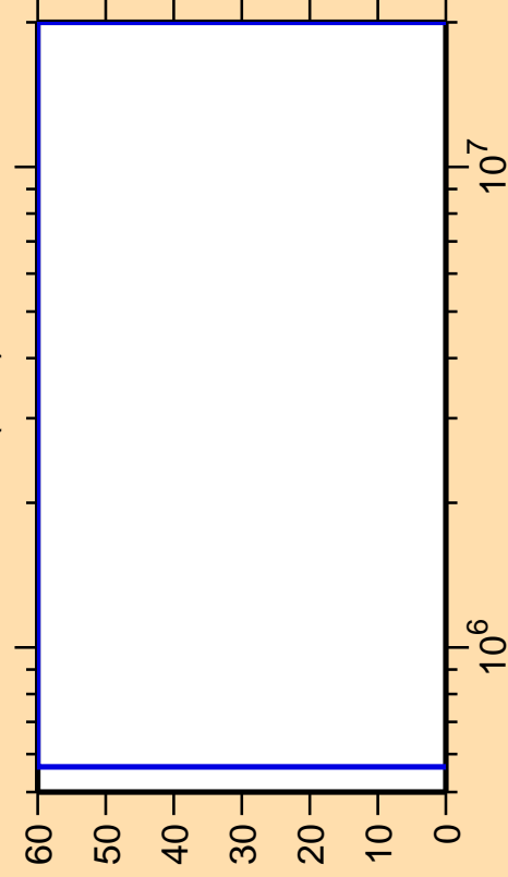
\Delta\sigma/\sigma vs. E for ^{168}\text{Lu}(n,\alpha)
