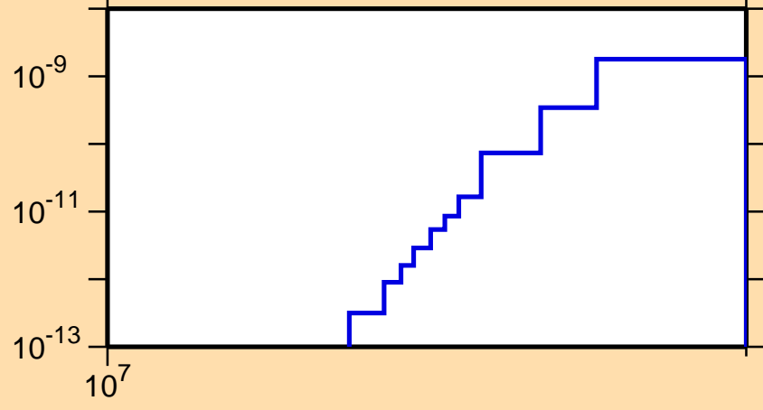
\sigma vs. E for ^{168}\text{Lu}(\text{mt } 45)
