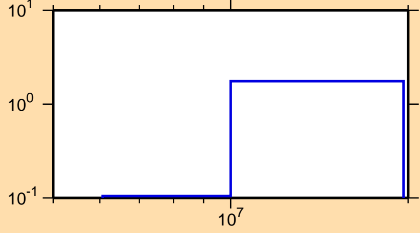
\sigma vs. E for ^{168}\text{Lu}(n,2n)
