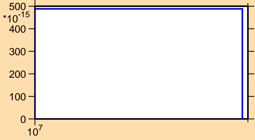
\sigma vs. E for ^{168}\text{Lu}(n,pd)
