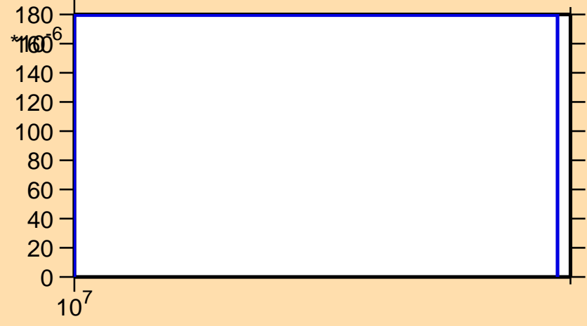
\sigma vs. E for ^{168}\text{Lu}(n,3n)
