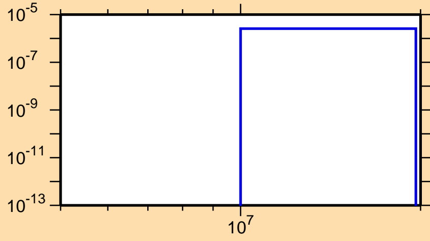
\sigma vs. E for ^{168}\text{Lu}(n,2n\alpha)
