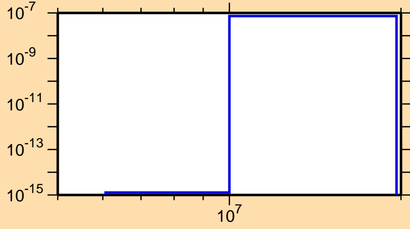
\sigma vs. E for ^{168}\text{Lu}(n,\text{He3})
