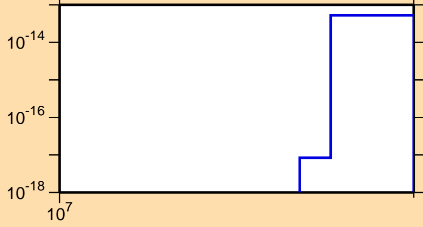
\sigma vs. E for ^{169}\text{Lu} (mt 34)
