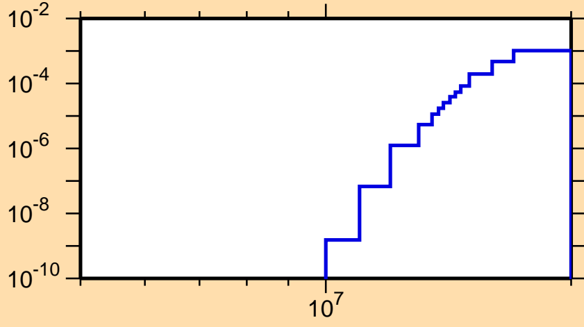
\sigma vs. E for ^{169}\text{Lu}(n,t)
