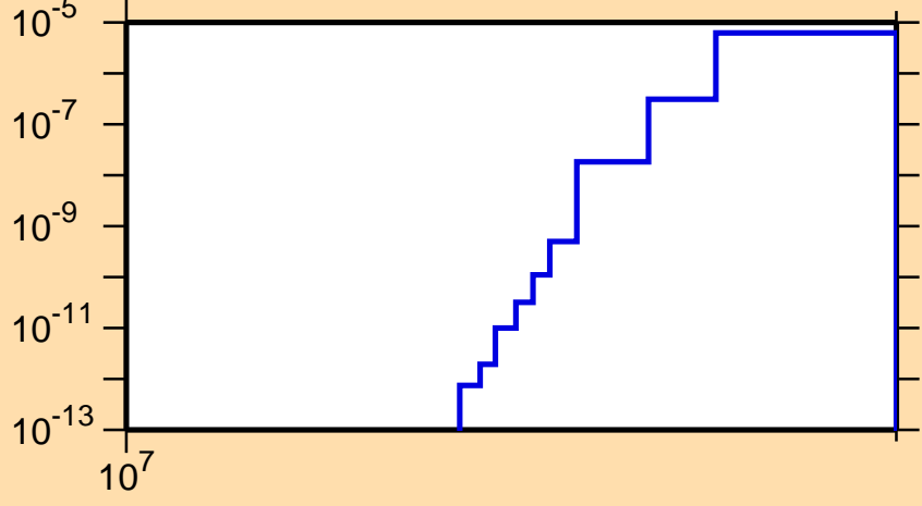
\sigma vs. E for ^{169}\text{Lu}(n,nd)
