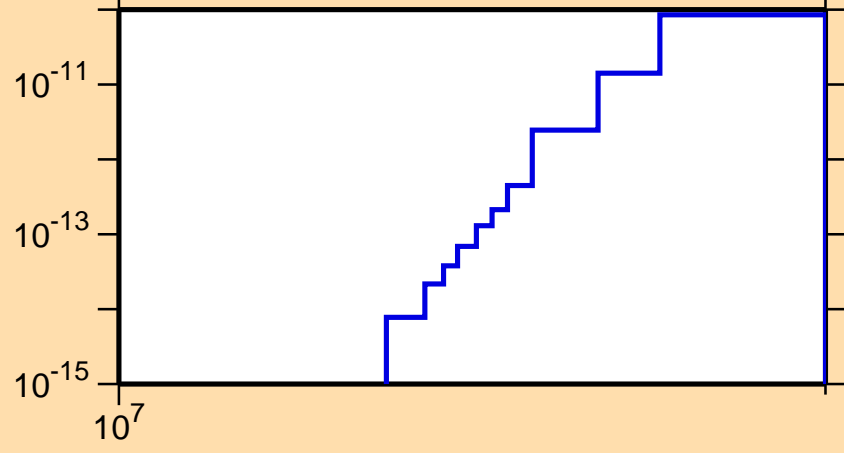
\sigma vs. E for ^{169}\text{Lu}(\text{mt117})
