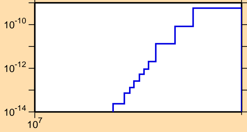
\sigma vs. E for ^{169}\text{Lu} (mt 45)
