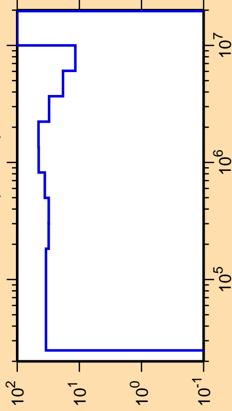
\Delta\sigma/\sigma vs. E for ^{169}\text{Lu}(n,\text{inel.})
