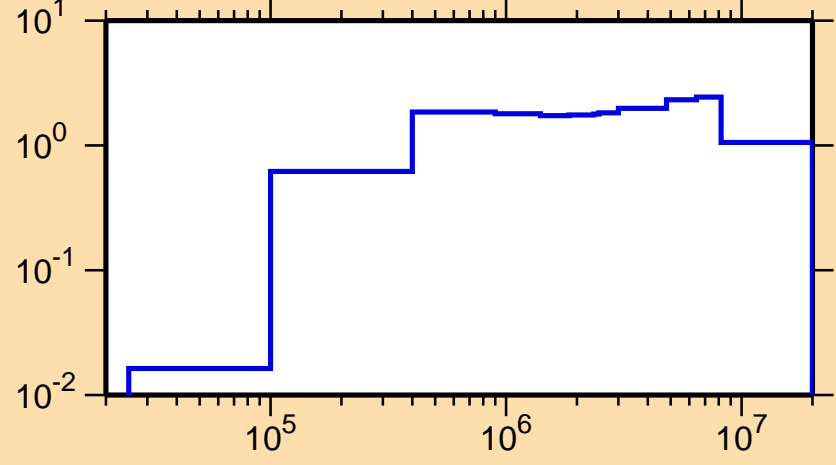
\sigma vs. E for ^{169}\text{Lu}(n,\text{inel.})
