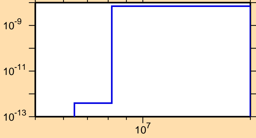
\sigma vs. E for ^{169}\text{Lu}(n,p\alpha)
