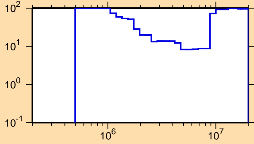
\Delta\sigma/\sigma vs. E for ^{169}\text{Lu}(n,n\text{cont.})
