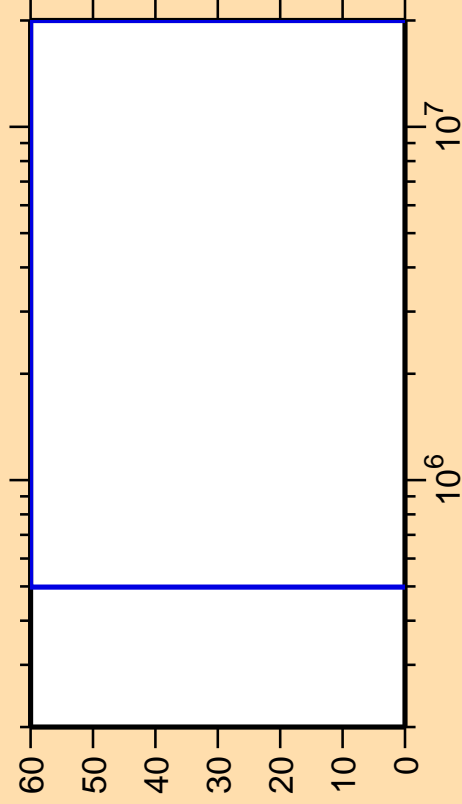
\Delta\sigma/\sigma vs. E for ^{169}\text{Lu}(n,\alpha)
