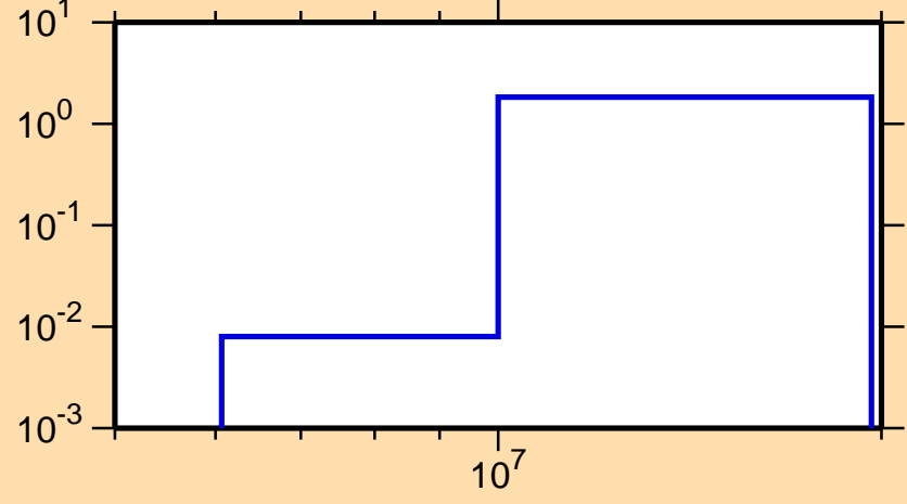
\sigma vs. E for ^{169}\text{Lu}(n,2n)
