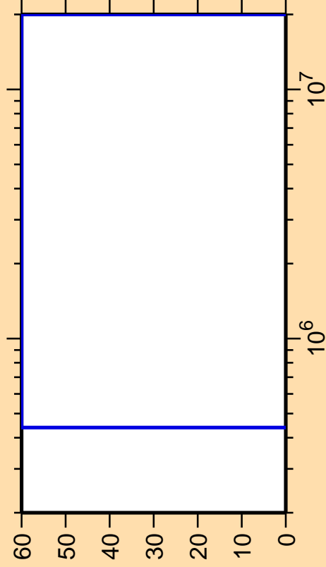
\Delta\sigma/\sigma vs. E for ^{170}\text{Lu}(n,\alpha)
