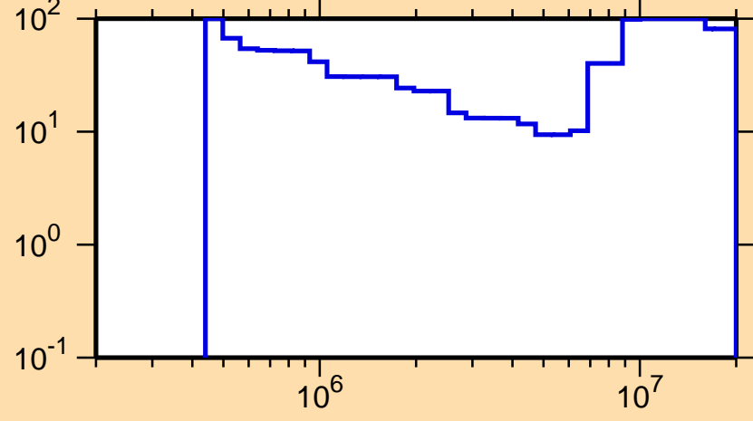
\Delta\sigma/\sigma vs. E for ^{170}\text{Lu}(n,n\text{cont.})
