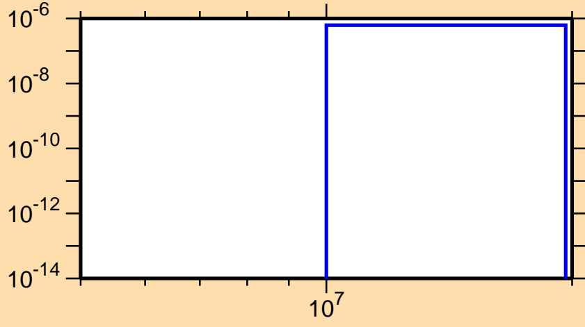
\sigma vs. E for ^{170}\text{Lu}(n,2n\alpha)
