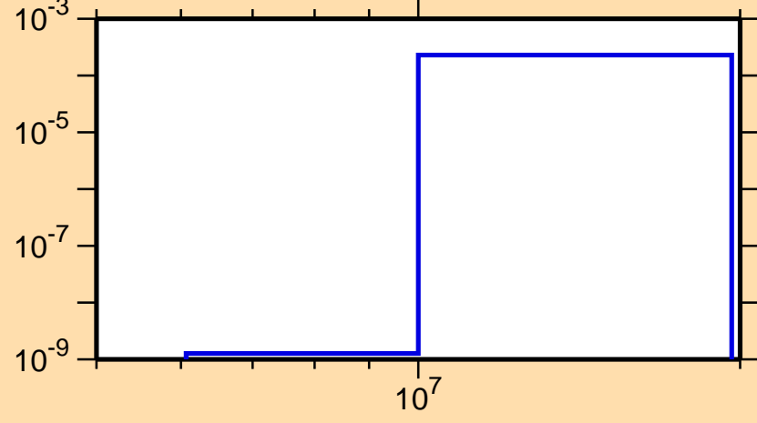
\sigma vs. E for ^{170}\text{Lu}(n,t)
