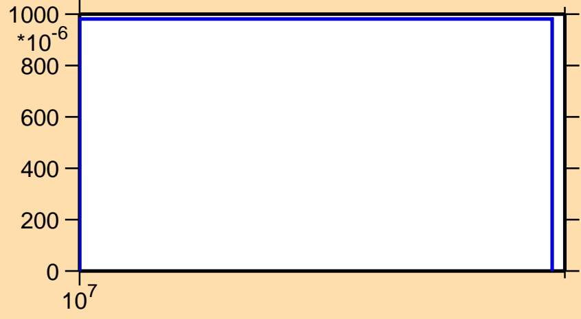
\sigma vs. E for ^{170}\text{Lu}(n,3n)
