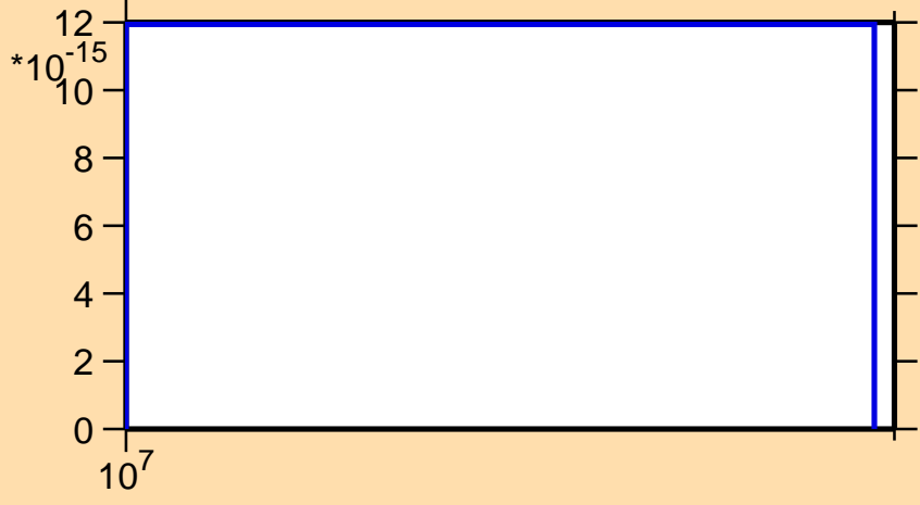
\sigma vs. E for ^{170}\text{Lu}(n,pd)
