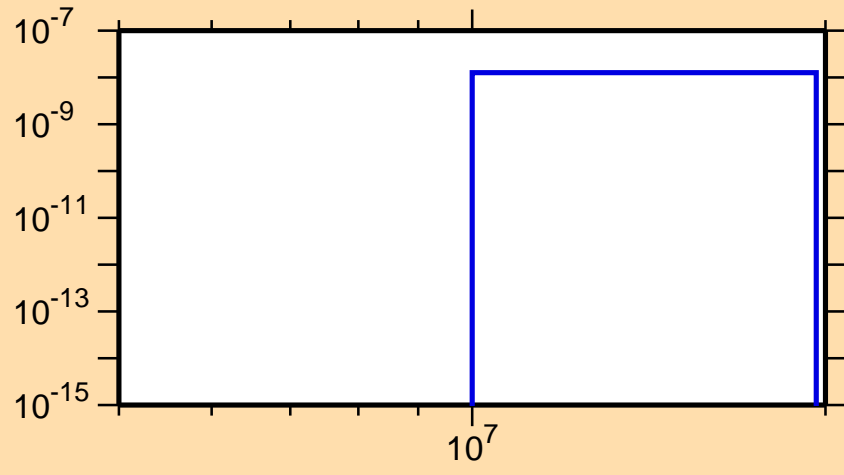
\sigma vs. E for ^{170}\text{Lu}(n,\text{He3})
