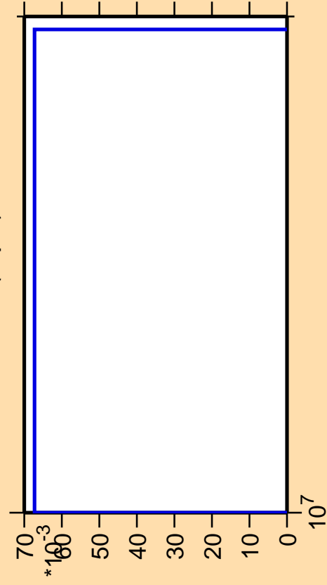
\Delta\sigma/\sigma vs. E for ^{170}\text{Lu}(n,pd)
