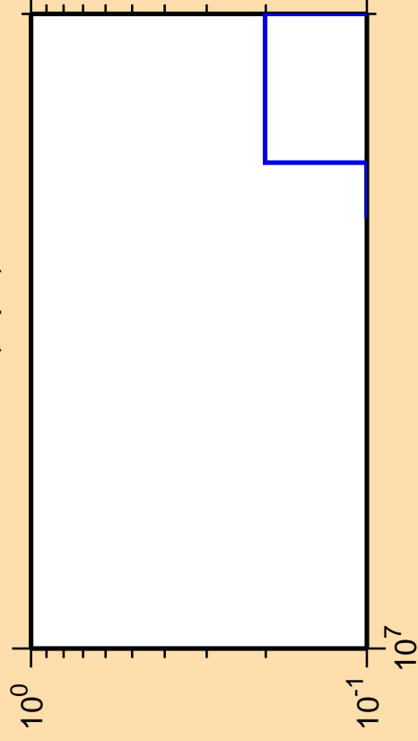
\Delta\sigma/\sigma vs. E for ^{171}\text{Lu}(n,pd)
