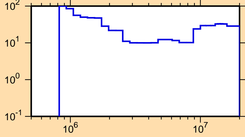
\Delta\sigma/\sigma vs. E for ^{171}\text{Lu}(n,n\text{cont.})
