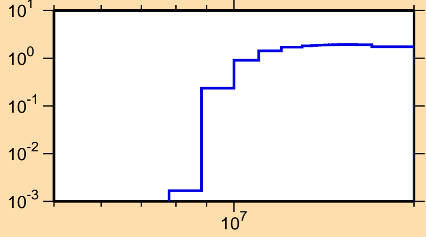
\sigma vs. E for ^{171}\text{Lu}(n,2n)
