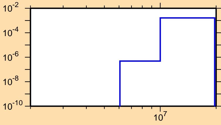
\sigma vs. E for ^{171}\text{Lu}(n,d)
