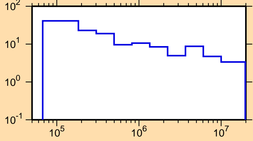
\Delta\sigma/\sigma vs. E for ^{171}\text{Lu}(n,\text{tot.})
