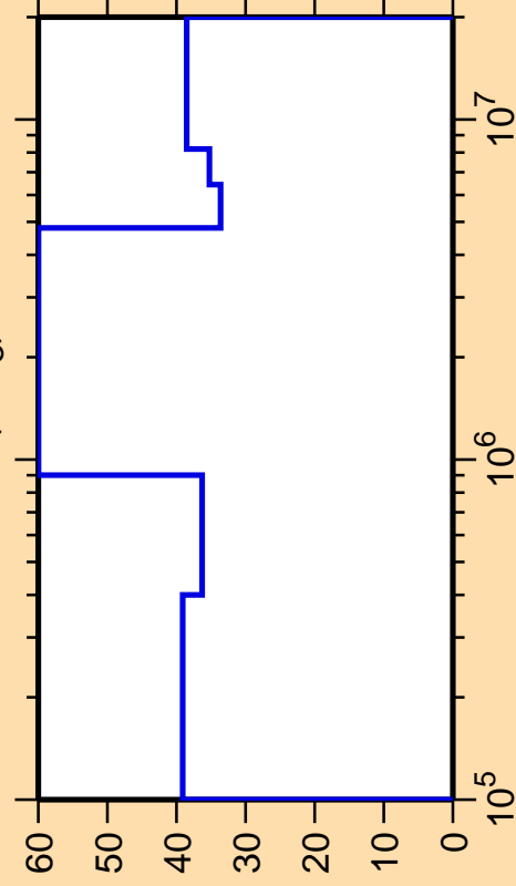
\Delta\sigma/\sigma vs. E for ^{171}\text{Lu}(n,n_3)
