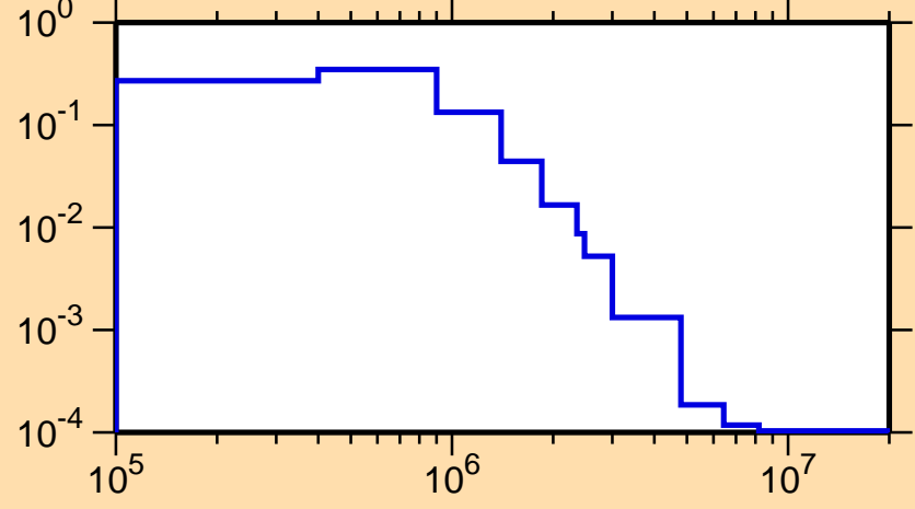
\sigma vs. E for ^{171}\text{Lu}(n,n_3)
