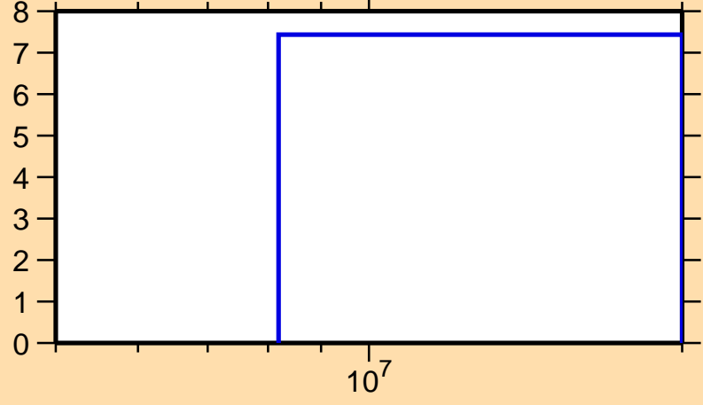
\Delta\sigma/\sigma vs. E for ^{171}\text{Lu}(n,\text{el.})
