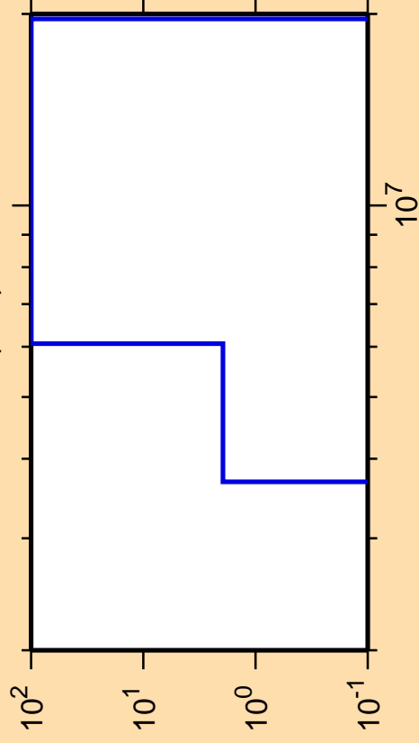
\Delta\sigma/\sigma vs. E for ^{171}\text{Lu}(n,d)
