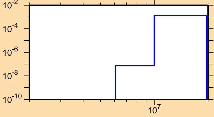
\sigma vs. E for ^{171}\text{Lu}(n,d)
