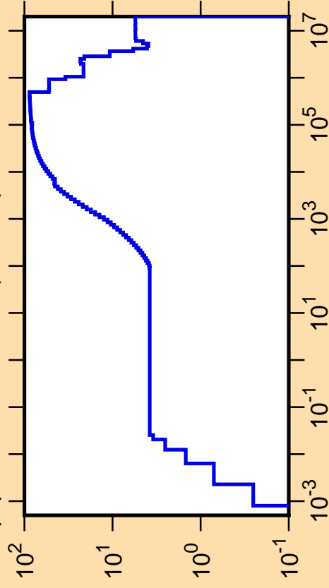
\Delta\mu/\mu vs. E for ^{172}\text{Lu}(\text{mt251})
