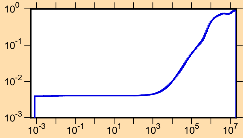
\mu vs. E for ^{172}\text{Lu}(\text{mt251})
