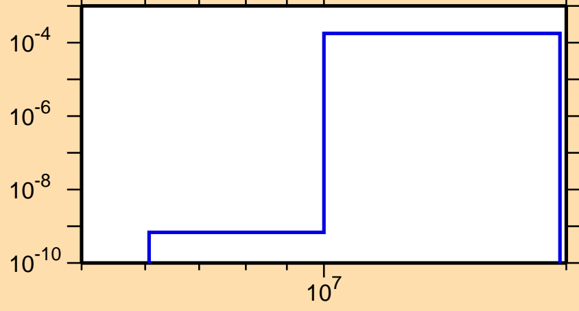
\sigma vs. E for ^{172}\text{Lu}(n,t)
