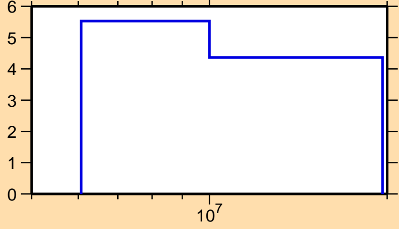
\Delta\sigma/\sigma vs. E for ^{172}\text{Lu}(n,\text{nonel.})
