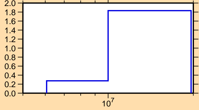
\sigma vs. E for ^{172}\text{Lu}(n,2n)
