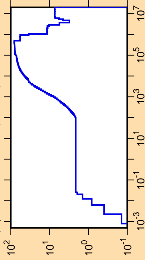
\Delta\mu/\mu vs. E for ^{173}\text{Lu}(\text{mt251})
