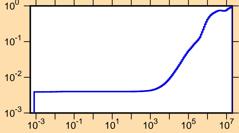
\mu vs. E for ^{173}\text{Lu}(\text{mt251})
