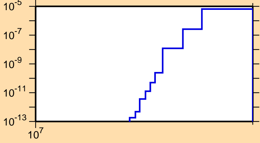
\sigma vs. E for ^{173}\text{Lu}(n,nd)
