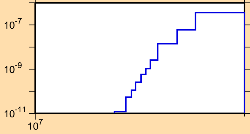
\sigma vs. E for ^{173}\text{Lu}(n,2n\alpha)
