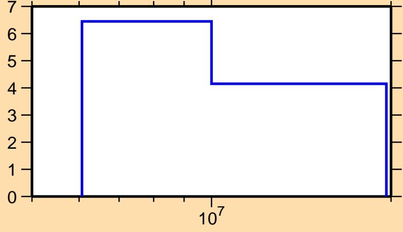
\Delta\sigma/\sigma vs. E for ^{173}\text{Lu}(n,\text{tot.})
