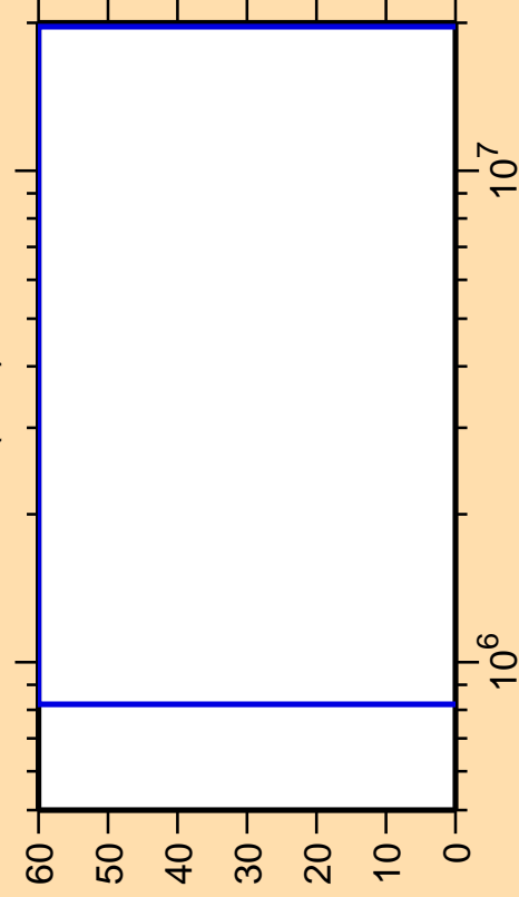
\Delta\sigma/\sigma vs. E for ^{173}\text{Lu}(n,\alpha)
