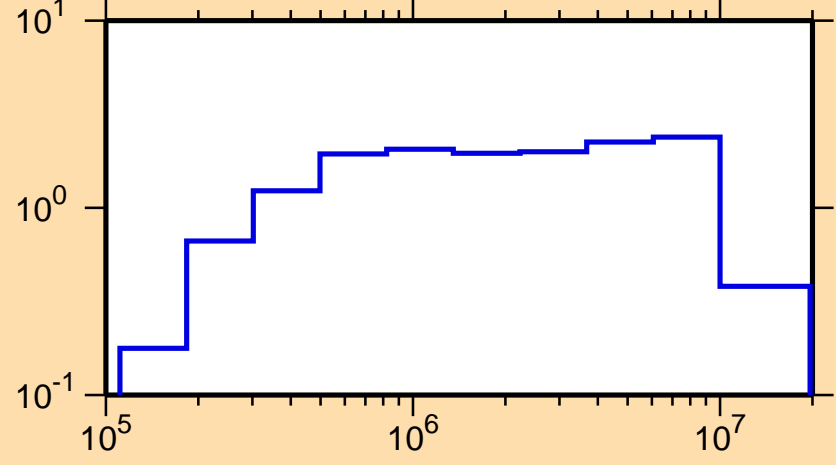
\sigma vs. E for ^{173}\text{Lu}(n,\text{inel.})
