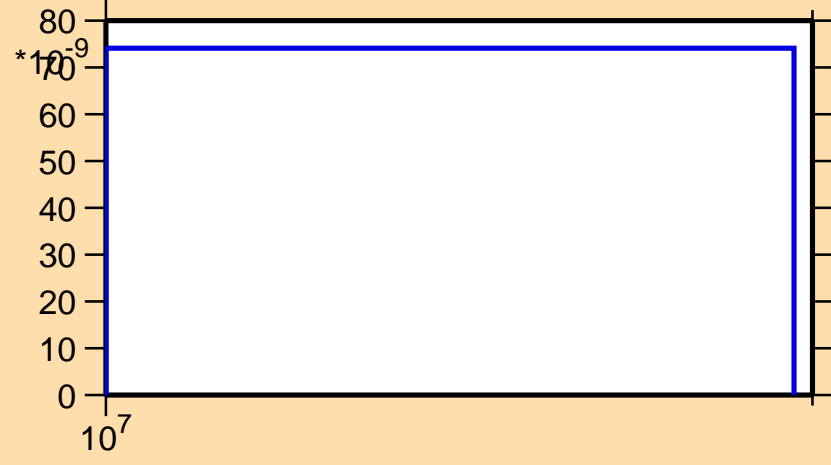
\sigma vs. E for ^{173}\text{Lu}(n,\text{nd})
