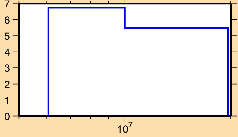
\Delta\sigma/\sigma vs. E for ^{173}\text{Lu}(n,\text{nonel.})
