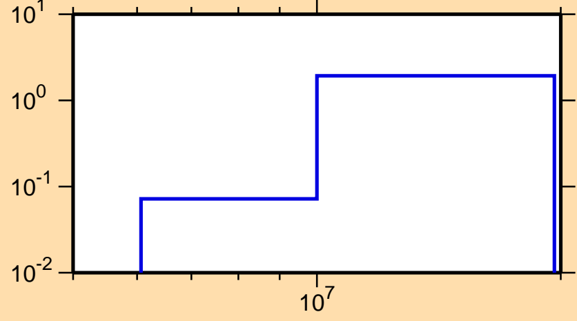
\sigma vs. E for ^{173}\text{Lu}(n,2n)
