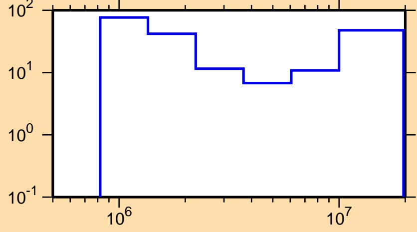
\Delta\sigma/\sigma vs. E for ^{173}\text{Lu}(n,n\text{cont.})
