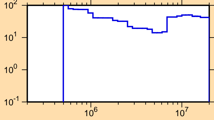
\Delta\sigma/\sigma vs. E for ^{174}\text{Lu}(n,n\text{cont.})
