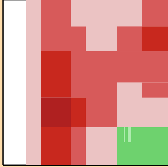
\Delta\sigma/\sigma vs. E for ^{174}\text{Lu}(n,2n)
