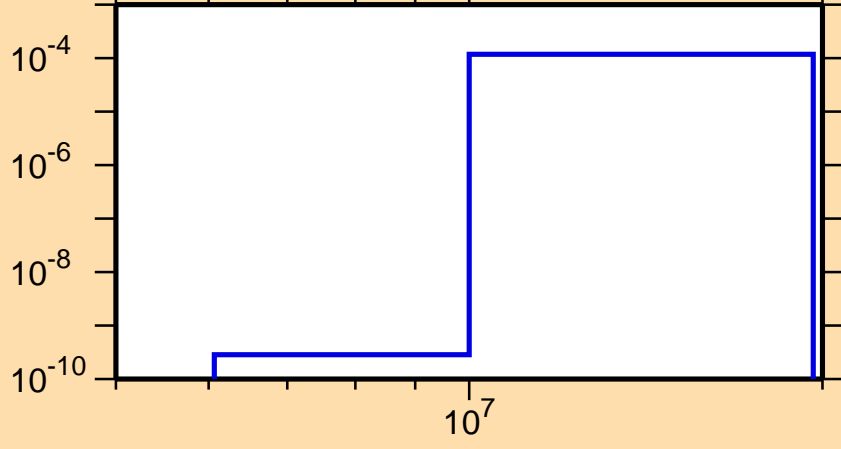
\sigma vs. E for ^{174}\text{Lu}(n,t)
