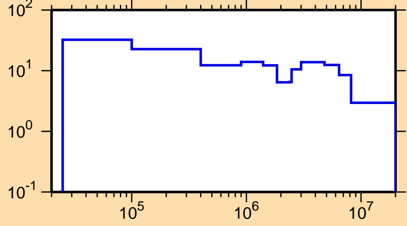
\Delta\sigma/\sigma vs. E for ^{174}\text{Lu}(n,\text{tot.})
