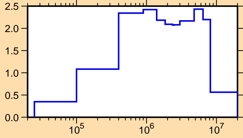
\sigma vs. E for ^{174}\text{Lu}(n,\text{inel.})
