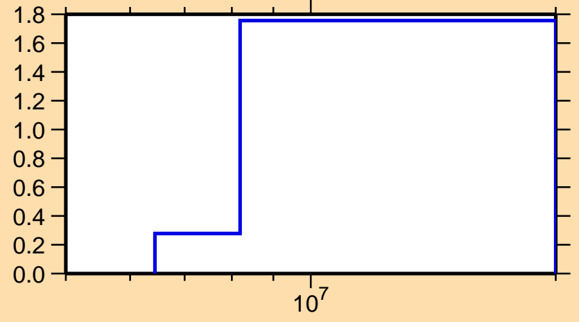
\sigma vs. E for ^{174}\text{Lu}(n,2n)
