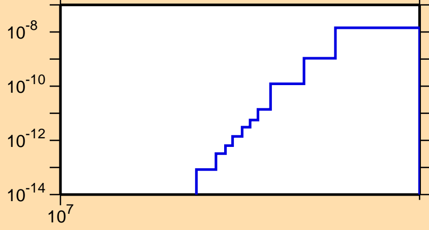
\sigma vs. E for ^{174}\text{Lu}(n,\text{He3})
