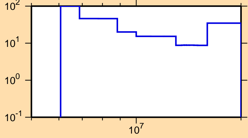
\Delta\sigma/\sigma vs. E for ^{174}\text{Lu}(n,2n)
