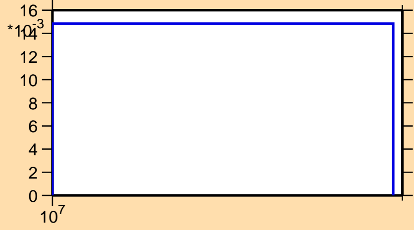
\sigma vs. E for ^{174}\text{Lu}(n,3n)
