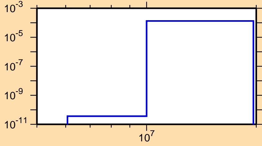
\sigma vs. E for ^{174}\text{Lu}(n,t)
