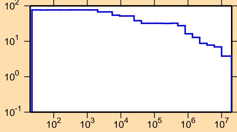
\Delta\sigma/\sigma vs. E for ^{174}\text{Lu}(n,\text{nonel.})
