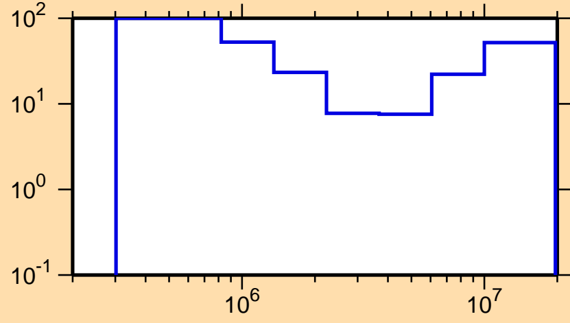
\Delta\sigma/\sigma vs. E for ^{174}\text{Lu}(n,n\text{cont.})
