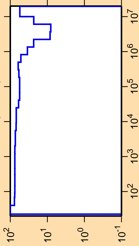
\Delta\sigma/\sigma vs. E for ^{174}\text{Lu}(n,\text{inel.})
