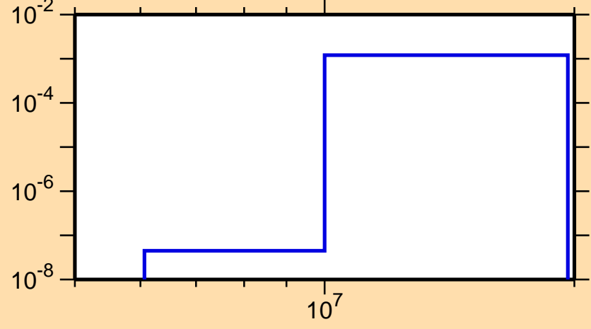
\sigma vs. E for ^{174}\text{Lu}(n,d)
