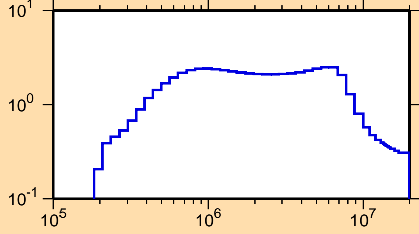
\sigma vs. E for ^{176}\text{Lu}(n,\text{inel.})
