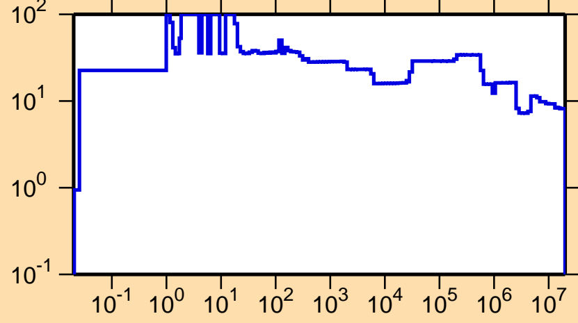
\Delta\sigma/\sigma vs. E for ^{176}\text{Lu}(n,\text{nonel.})
