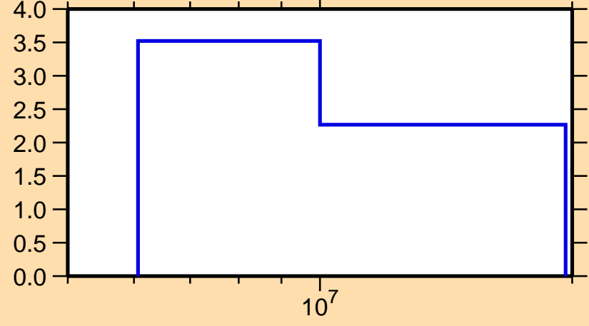
\Delta\sigma/\sigma vs. E for ^{176}\text{Lu}(n,\text{tot.})
