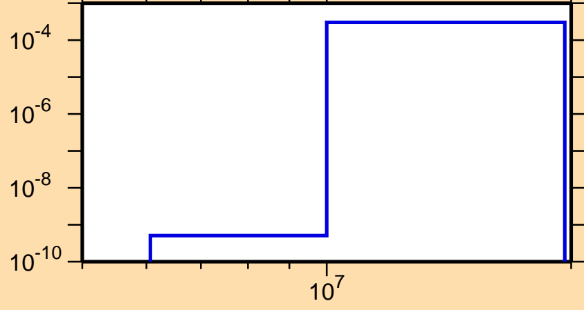
\sigma vs. E for ^{176}\text{Lu}(n,t)
