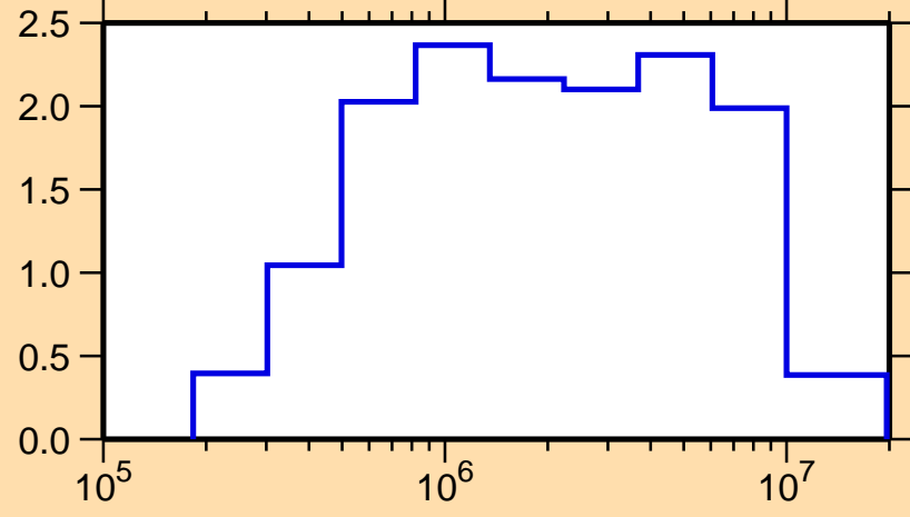
\sigma vs. E for ^{176}\text{Lu}(n,\text{inel.})
