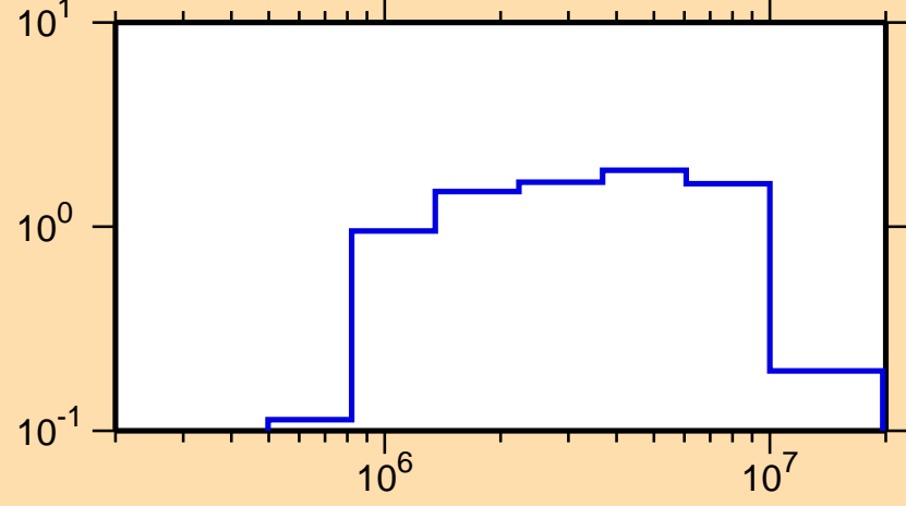
\sigma vs. E for ^{176}\text{Lu}(n,n\text{cont.})
