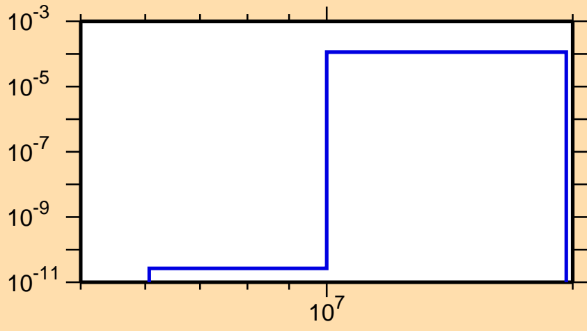
\sigma vs. E for ^{176}\text{Lu}(n,t)
