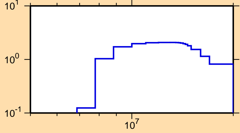
\sigma vs. E for ^{177}\text{Lu}(n,2n)
